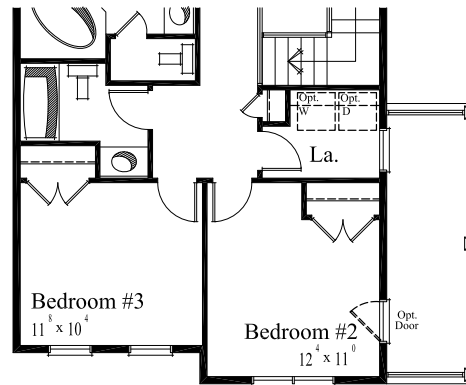
PART. THIRD FLOOR PLAN
