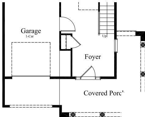
PART. FIRST FLOOR PLAN
