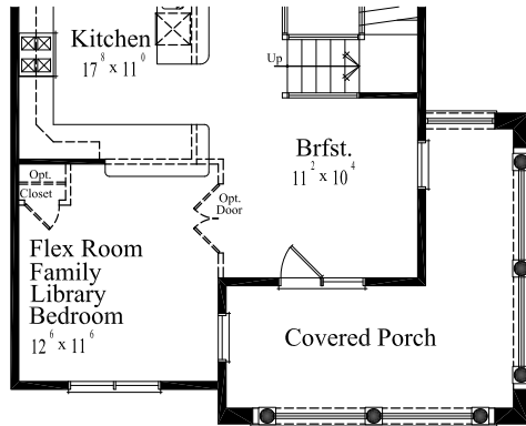
PART. SECOND FLOOR PLAN
